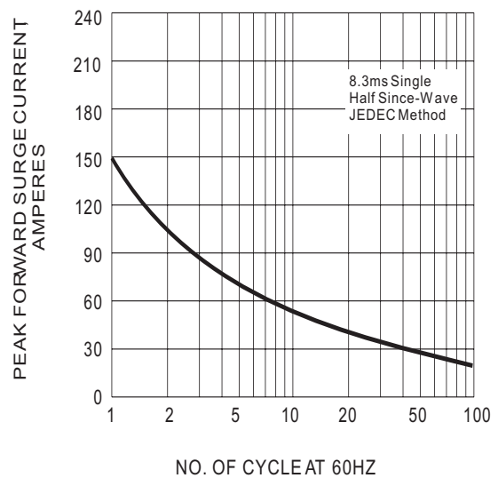
Fig.4- TMAXIMUM NON - REPETITIVE SURGE CURRENT
