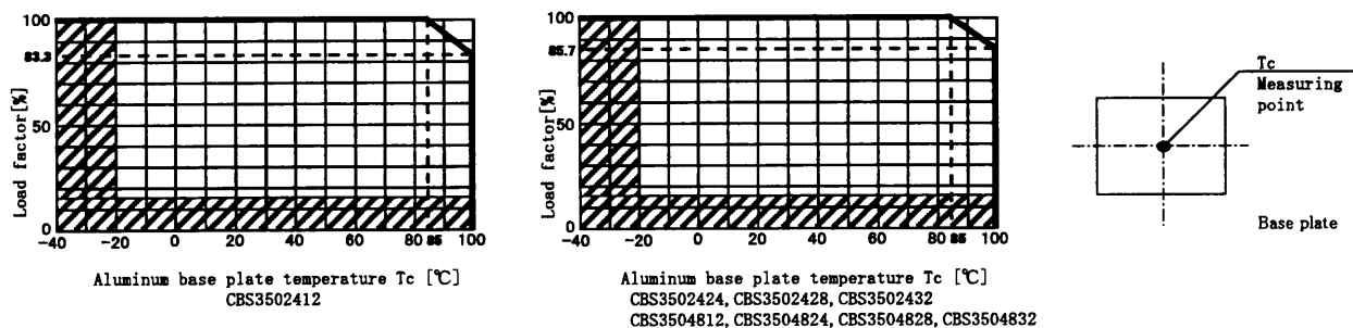
Fig. 2.1 CBS350 Derating curve and measuring point
