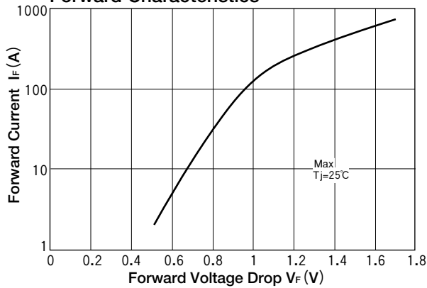
Forward Characteristics
